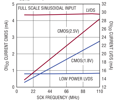
OV_{DD} Current vs SCK Frequency, C_{LOAD} = 10\text{pF}
