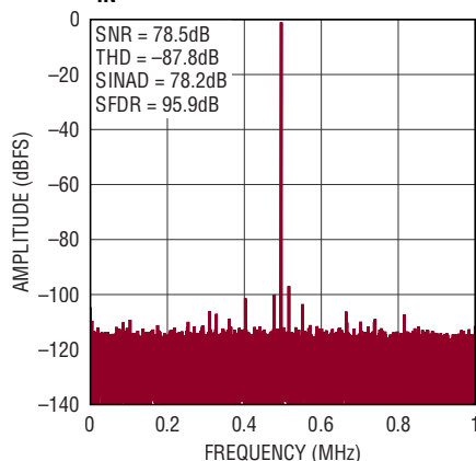
32k Point FFT, f_{\text{SAMPL}} = 2\text{Msps} , f_{\text{IN}} = 500\text{kHz}
